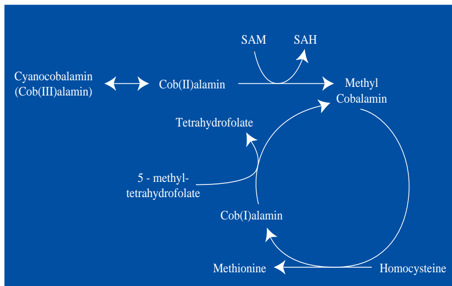
Figure 3. Methylcobalamin Metabolism
